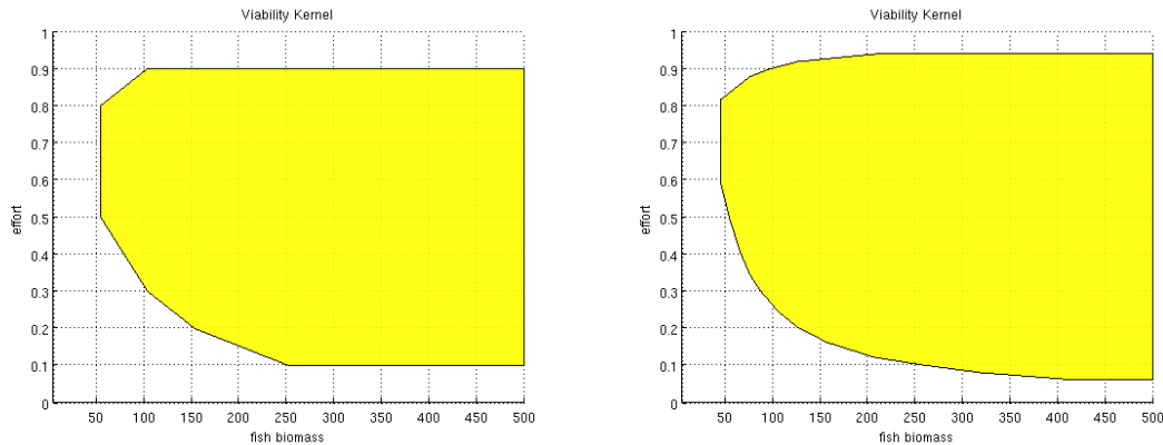
(A) An interpolation of the viability domain for FisheriesControl using \delta = 11 in each dimension.
