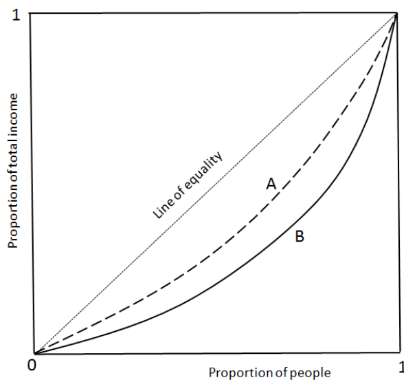
Figure 1: Two Lorenz Curves
