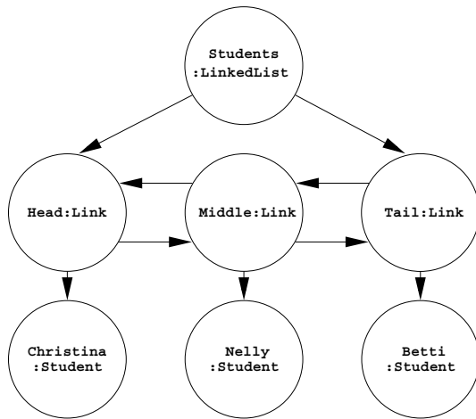
Figure 1. Simple object graph of a linked list
