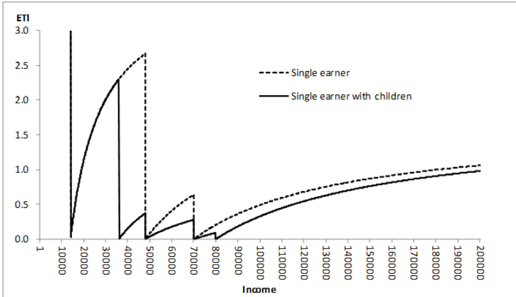
Figure 5: Revenue-Maximising Elasticities
